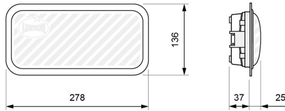
Watertight housing
