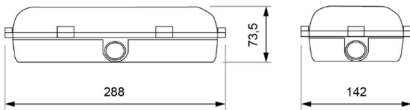
Watertight housing
